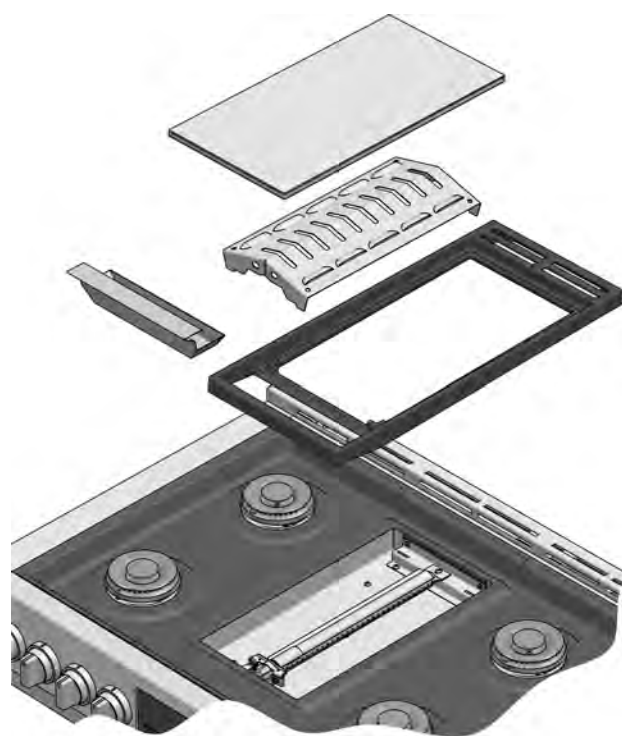
EXPLODED VIEW OF BURNER GRIDDLE
